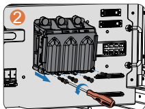
2 Remove the screws from the box
