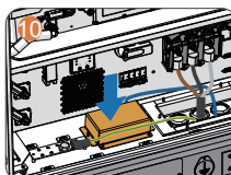
10 Install the protective cover
