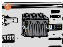
1 Release the snap-fits on the junction box
