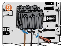
9 Secure the snap-fits and tighten the screws
