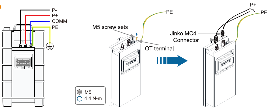
Connection Diagram
