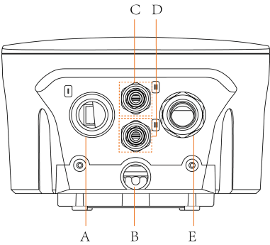
figure 1-2 Port Diagram
