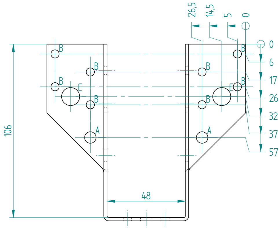
Product name: Joist hanger 48x106 Material: HDG DX51D Z275
