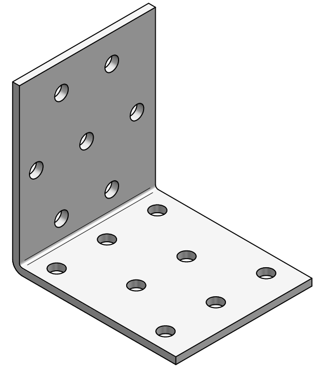
Product name: Angle bracket 60x60x50x2,5 Material: HDG DX51D Z275
