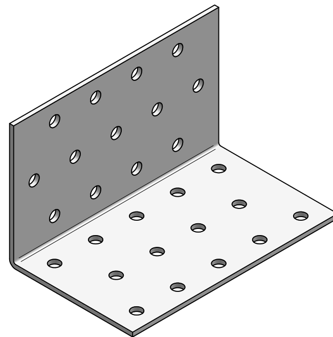
Product name: Angle bracket 60x60x100x2,0 Material: HDG DX51D Z275
