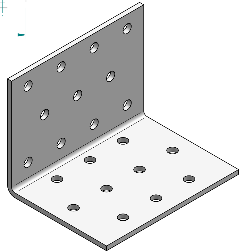
Product name: Angle bracket 60x60x80x2,5 Material: HDG DX51D Z275
