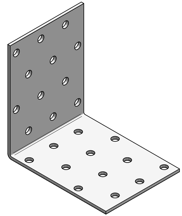
Product name: Angle bracket 80x80x60x2,0 Material: A2 AISI304
