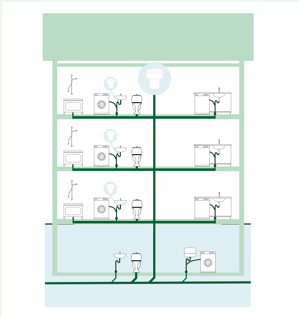
Ventilated stack – Connected appliances
