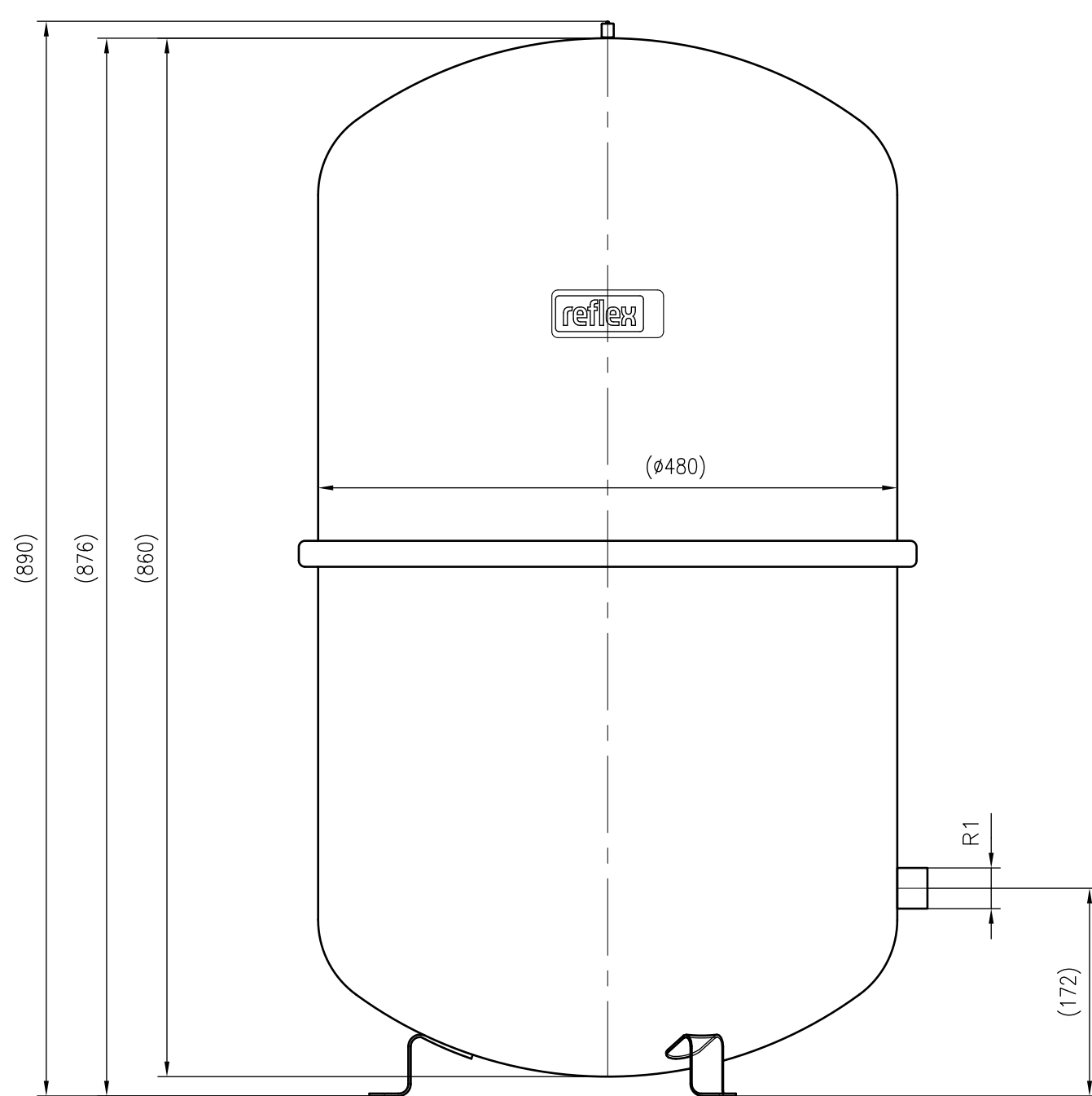
Front view
