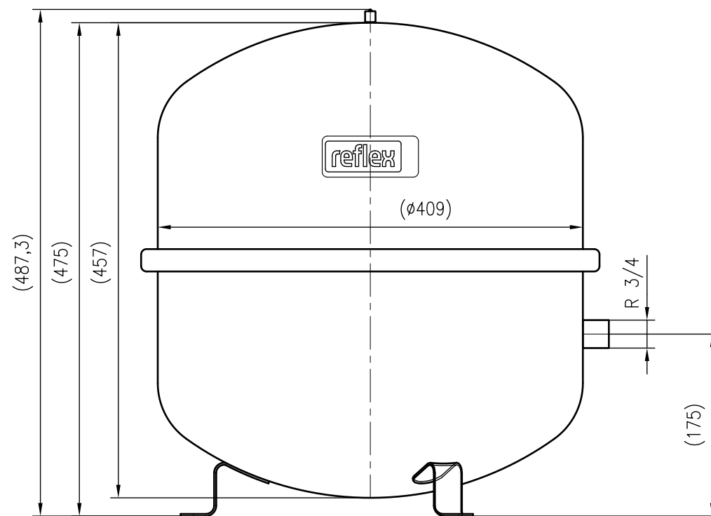
Front view
